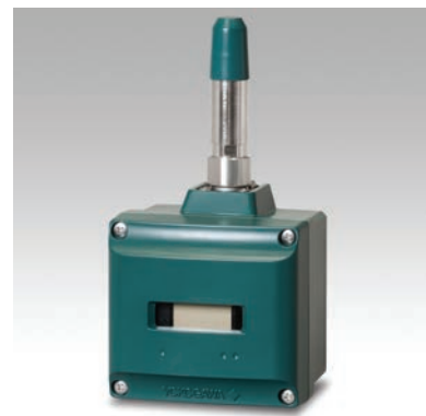
Fig.5. Yokogawa's multi-function wireless adaptor enables wired devices that transmit and receive digital on/off signals or receive 4–20 mA analogue signals to function as ISA100 Wireless™ field wireless devices
