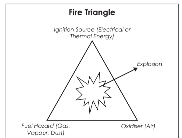
Figure 2. An explosion is any uncontrolled propagation of a combustion wave. To create an explosion there has to be fuel (i.e., an explosive gas such as hydrogen), an oxidiser (such as the oxygen in air) and a source of ignition energy (i.e., a hot surface or an electrical spark). Once the mechanism to mix the fuel and the oxidiser exists, the resulting explosion is commonly represented in 'the fire triangle' shown here.
