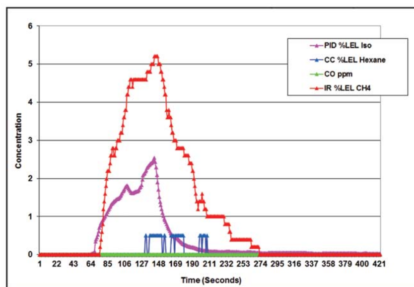
Figure 3: Response of PID, pellistor type LEL and NDIR combustible gas sensors to warm 130°F (54°C) diesel vapor. Readings for all three sensors displayed on LEL scale. PID and IR LEL sensor show strong response. Pellistor LEL sensor shows almost no response.
