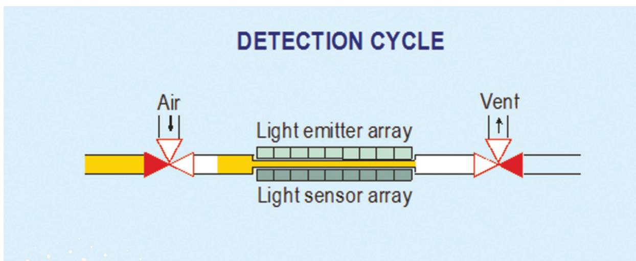
The working principle of D7945, in which a fixed volume of test fuel is driven by a calibrated air pressure force across timed segments of a horizontal capillary tube. The times of transit of the sample can then be used to calculate its viscosity according to the Hagen-Poiseuille law.
