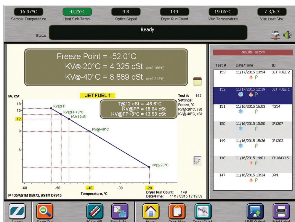
An illustrative output of the JFA-70Xi test screen showing various results. In particular, the 12 mm 2 /s temperature is reported if it is found to be warmer than the freezing point, since the fuel is free of solids when 12 mm 2 /s is reached.
