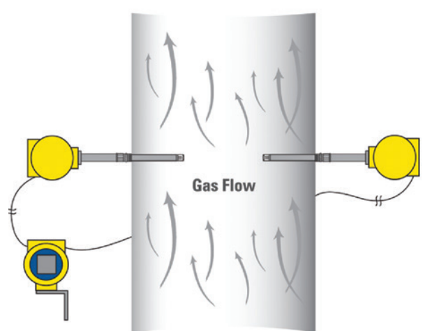
Figure 3: Dual Element ST102 Flow Meter
